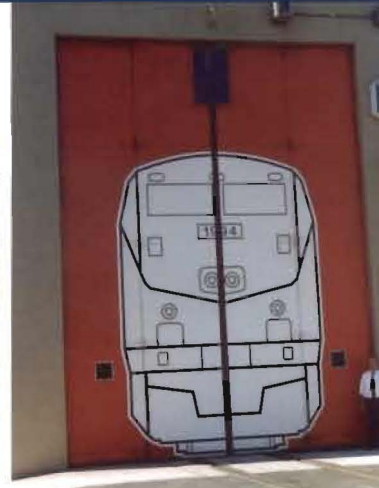
Right: Four Fold Catenary Transportation Door installed at Amtrak, Boston, MA. There are no floor guides making EPD high-cycle Four Fold Doors perfect for transportation. Doors open and close at a speed of two feet per second, and can be operated manually in case of a power failure.
